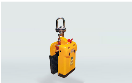
ABACO Little Giant slab lifter
